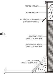
TYPICAL FLASHING DETAIL
